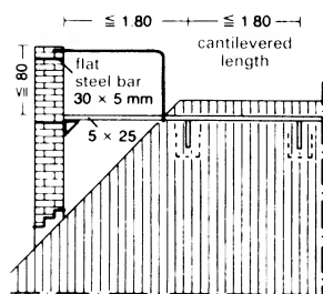
13 Length and attachment of the crawling board
